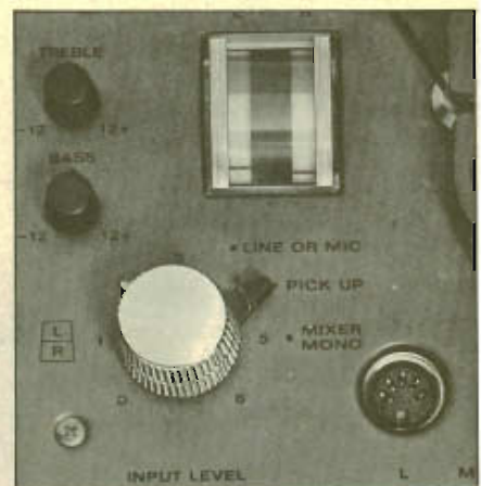
Bass and treble continuously variable within ± 12 dB. 2 input level controls for mixing in mono. Input selector for line/microphone and record player and mixing in mono. Model 1200X has amplifier for magnetic pickup.
