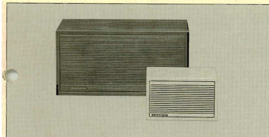
SEPARATE LOUDSPEAKER 9. A high quality remote loudspeaker for kitchen, sitting-room or sleeping-room. Dimensions: Length 16½", height 8½", depth 6". Volume: 8,5 litres. Teak cabinet.
