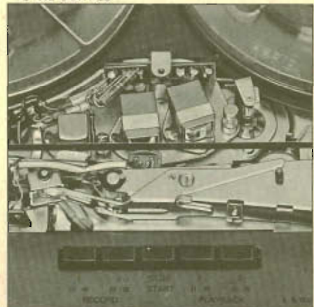
Separate heads for erasing, recording, playback and separate bias head, Tandberg made. (Cross-Field). By introducing the Cross Field technique Tandberg has reached sensational specifications for frequency range and signal/noise ratio.
